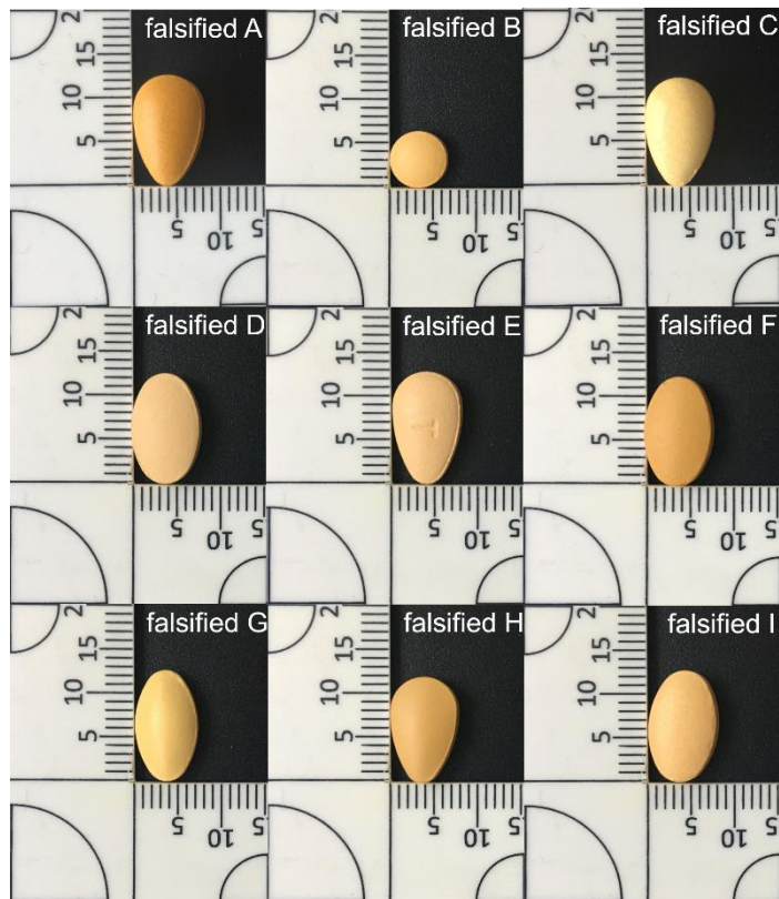
falsified Cialis
