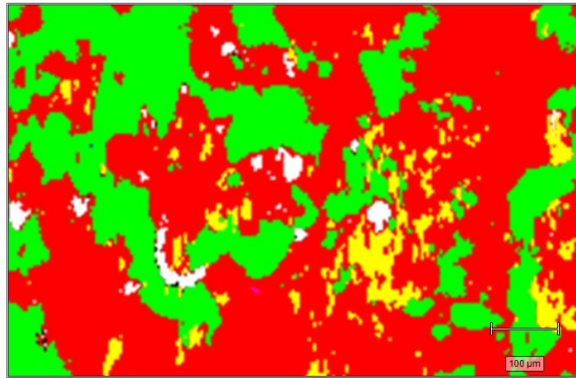
falsified G
