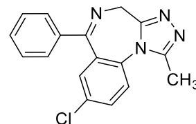
Alprazolam
