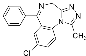
Alprazolam
