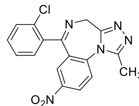
Clonazolam
