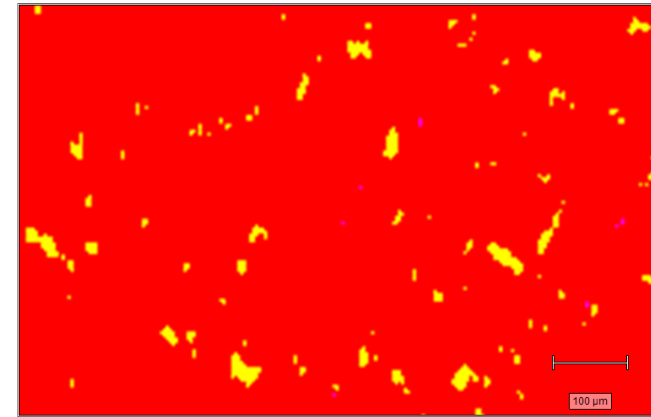
falsified C
