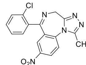
Clonazolam
