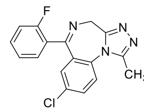
Flualprazolam
