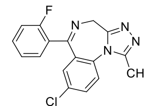
Flualprazolam
