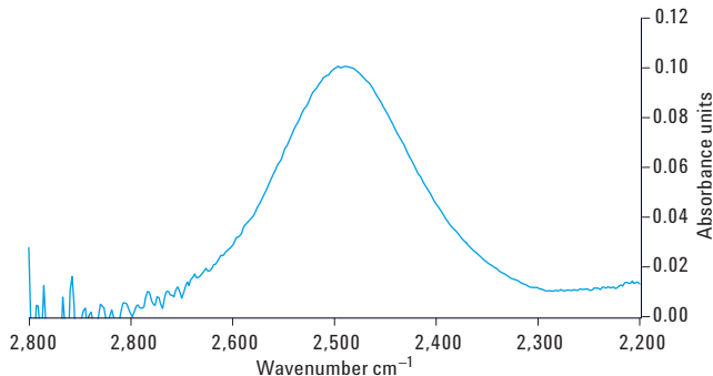
Figure 3. O-D absorbance band in spectrum measured with Agilent 4500 Series FTIR with 100- \mu\text{m} pathlength TumbIIR sample interface.
