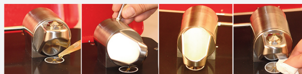
Figure 2. TumbIIR operation: Place sample on window; rotate second window into position; analyze sample; clean windows by wiping.
