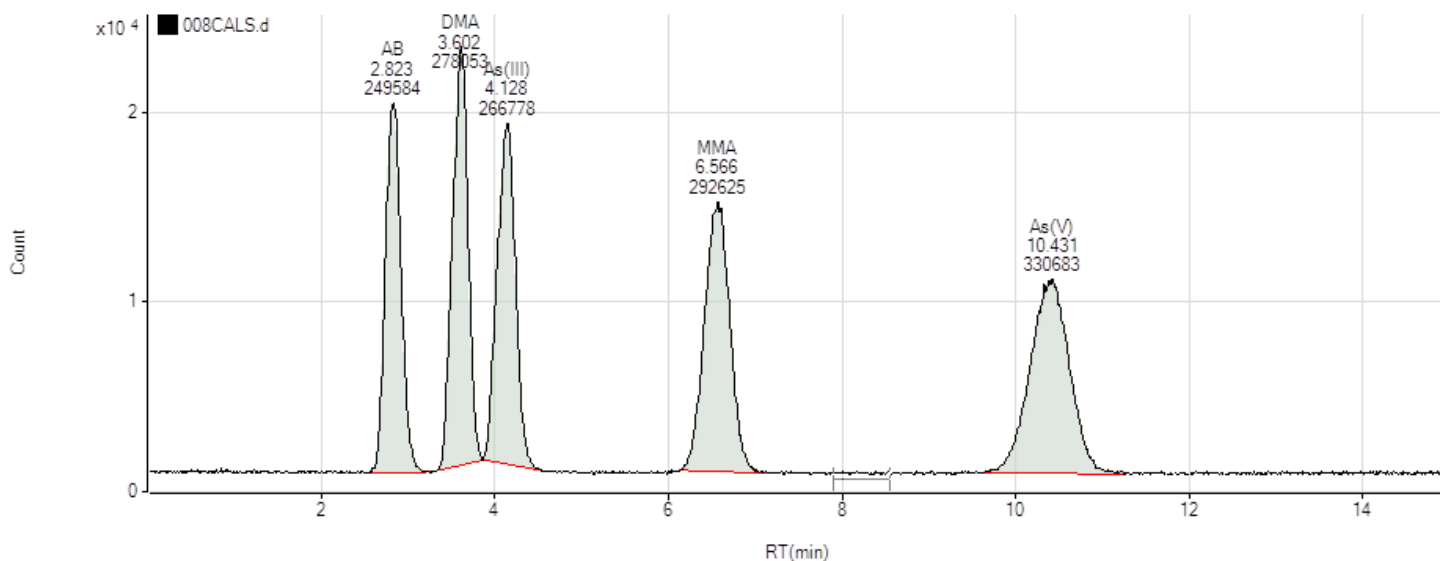
Figure 2. Chromatogram of 500 ng/L (ppt) mixed As species standard showing good sensitivity and peak separation, and noise region used for S/N and LOD calculation.
