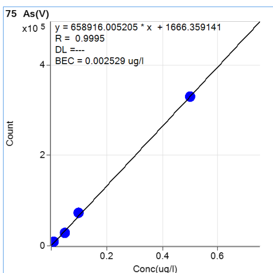
Figure 3. Calibration graphs for AB, DMA, As(III), MMA, and As(V).
