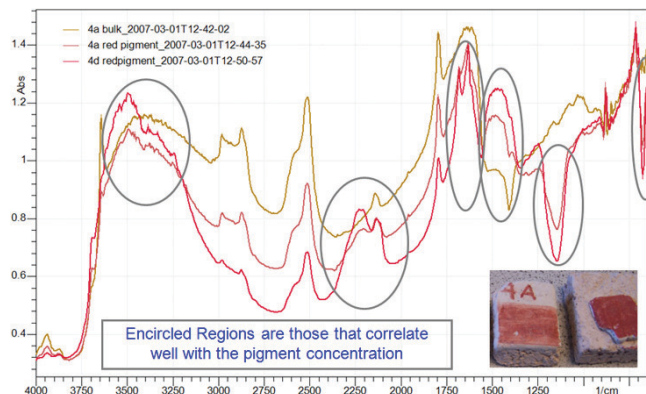
Figure 9. The infrared spectrum of carmine red pigment on stone correlates quite well with the amount of pigment on the surface and also shows the bands from the underlying stone matrix
