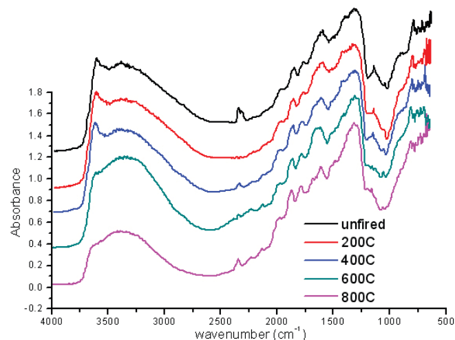
Figure 10. The changes in the diffuse reflectance spectra of clays correlate quite well with increasing firing temperature
