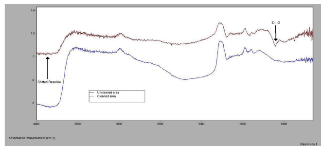
Figure 4. Uncleaned area of painting shows significant baseline shift due to dirt particles as well as the presence of silica on the surface. After the cleaning process, spectrum shows far less scattering and the silica particles have been removed.
