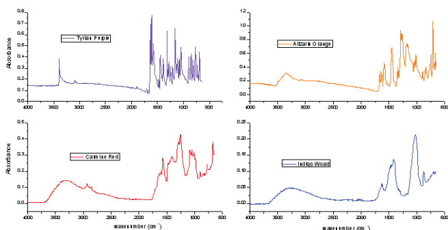
Figure 8. The infrared spectra of these common ancient pigments and dyes are rich in detail and are not affected by the issue of fluorescence, as in Raman spectroscopy. The Agilent 4100 ExoScan FTIR, equipped with a spherical ATR sampling accessory, makes non-destructive pigment analysis straightforward.
