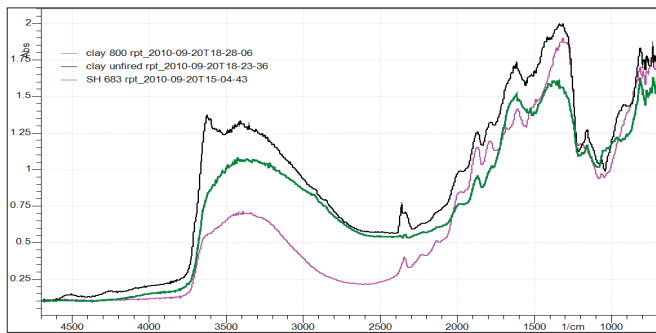
Figure 11. The infrared spectra of Orkney Island unfired clay and clay fired at 800 °C are compared to that of a clay fragment found at the site. The latter spectrum indicates that the pottery was fired at between 400 and 600 °C.
