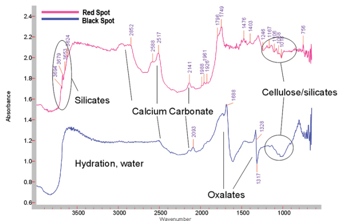
Figure 2. Infrared spectrum of the red and black areas of door showed varied levels of oxalate present
