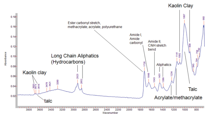
Figure 13. The infrared analysis of the lower leg of the “Dr J” mural recorded with the Agilent 4100 ExoScan FTIR shows spectral contributions from both the polymer coating and the underlying paint. By following changes in these bands, conservationists hope to be able to determine when restoration is required.
