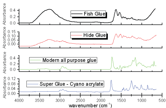
Figure 5. The infrared spectra of ancient, animal-based glues and modern synthetic glues are different and are strong indicators for type and time of material repair
